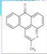
2-Methyl-naphtho[1,2,3-de]quinoline
